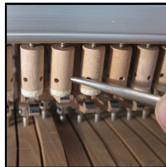
Adjusting letoff
